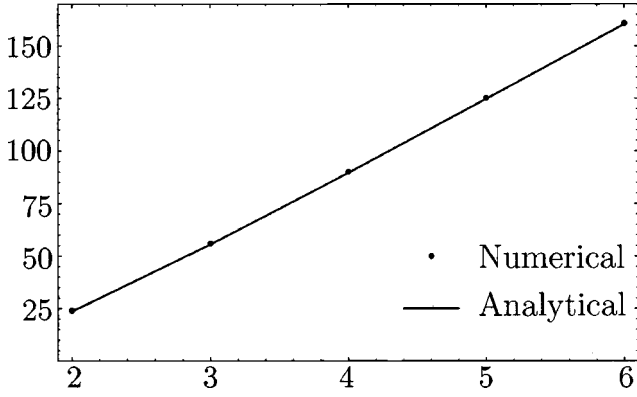
FIG. 8. Comparison between the BPS bound on the tunneling action from Eq. (50) (solid line) and the actual semiclassical tunneling action from the numerical calculation (dots). It is clear that the actual instanton configuration saturates the BPS bound.
