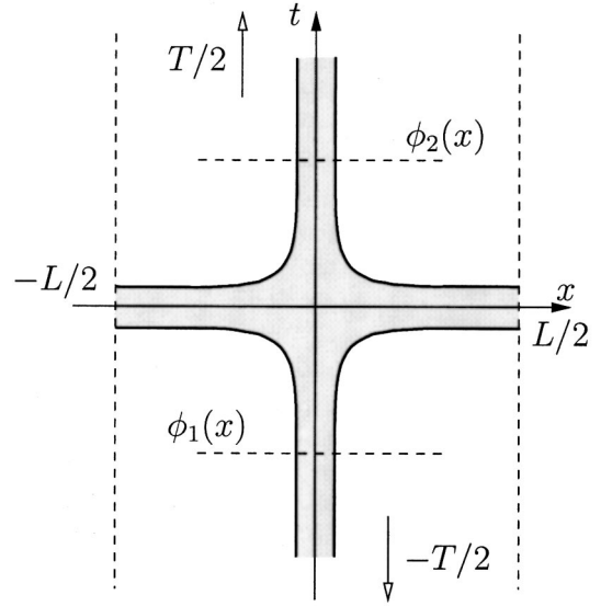
FIG. 3. The energy distribution corresponding to the interpolating configuration; the unshaded area has the “vacuum” energy density.
