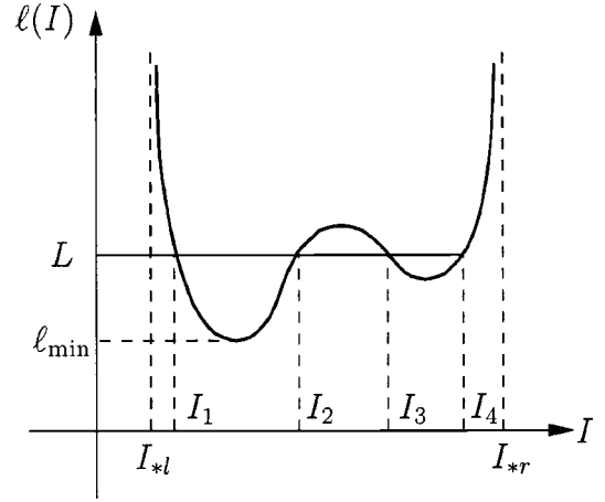
FIG. 2. The period function l versus I .
