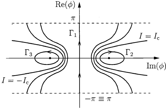
FIG. 4. The target space of the model. The three types of non-contractible cycles are indicated by \Gamma_1 and \Gamma_2 and \Gamma_3 .
