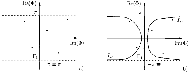
FIG. 1. (a) The general singularity structure of the quantity d\mathcal{W}/d\Phi in the complex \Phi plane; (b) the critical trajectories corresponding to infinite periods.
