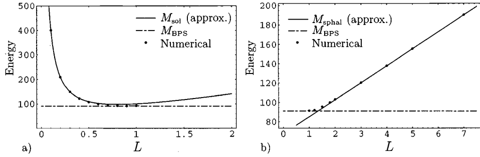
FIG. 5. (a) Energy of the real, non-BPS soliton as a function of the circumference L of the compact dimension; the BPS bound (dashed line), the analytical approximation M_{\text{sol}} = U + K for small L (solid line), and the actual numerically calculated soliton mass (dots) are shown. (b) Energy of the sphaleron, the real, unstable soliton for L > 1 as a function of the circumference L of the compact dimension; the BPS bound (dashed line), the linear analytical approximation for M_{\text{sphal}} for large L (solid line), and the actual numerically calculated sphaleron mass (dots) are shown.
