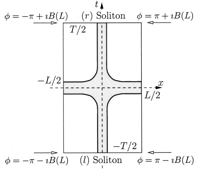
FIG. 6. Boundary conditions on the world sheet. The initial (l) and final (r) solitons are located at the bottom and top sides of the rectangle at t = -T/2 and t = T/2 , with the center of the energy density positioned at x = 0 . Periodic (modulo 2\pi ) boundary conditions apply to the left and right side of the rectangle. The shaded area significantly contributes to the action.
