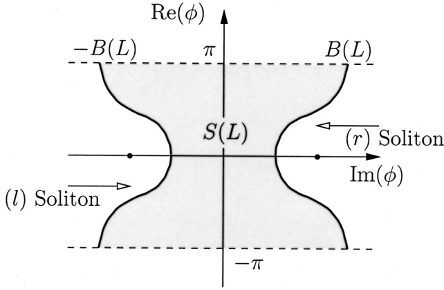
FIG. 7. The (r) and (l) solitons and the instanton in the complex \phi plane (compare Fig. 6 for the same configuration on the world sheet). The area S(L) is indicated by the shaded region.
